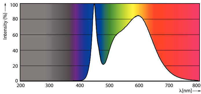
Spectral Power Distribution Colour - 150CC/LED/840/LS EX39 G2 BB 277-480V 3/1
