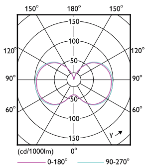
Light Distribution Diagram - 150CC/LED/840/LS EX39 G2 BB 277-480V 3/1
