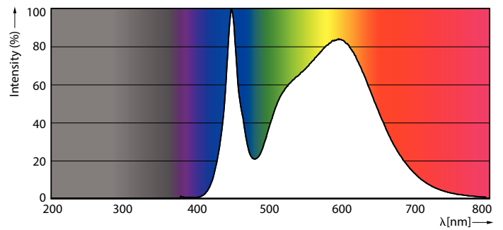
Spectral Power Distribution Colour - 450CC/LED/840/LS EX39 BB 3/1
