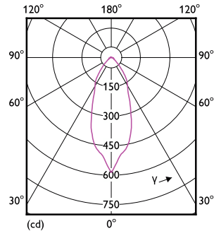
Light Distribution Diagram - MAS LEDspot VLE D 4.7-50W GU10 83036D5CT
