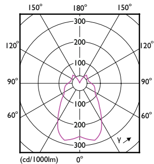
Light Distribution Diagram - MAS LEDlustre DT 2.8-25W E27 P48 CL
