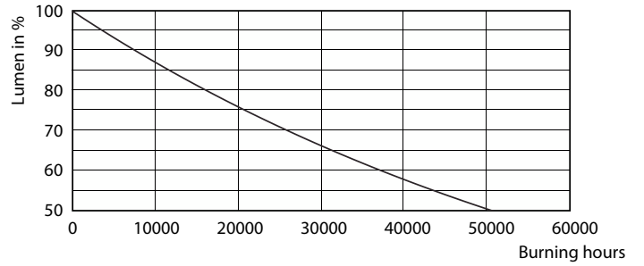
Lumen Maintenance Diagram - 7PAR20/LED/F40/830/E26/GL/DIM 120V
