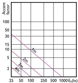
Accent Diagram - MAS LEDspot UE 2.4-50W GU10 ND 830 EELB
