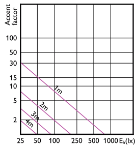
Accent Diagram - MAS LEDspot UE 2.4-50W GU10 ND 840 EELB
