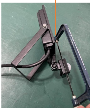
7. Saw off the sensor housing
