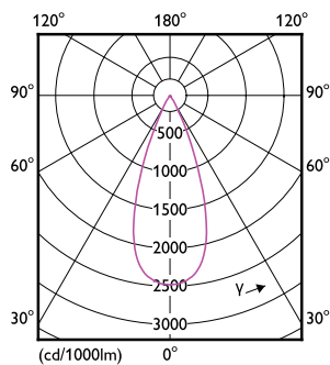
Light Distribution Diagram - RS350 G2 RC Rd D100 15W 40K 36D 1H
