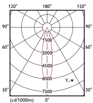
Light Distribution Diagram - RS350 G2 RC Rd D100 15W 30K 24D 1H
