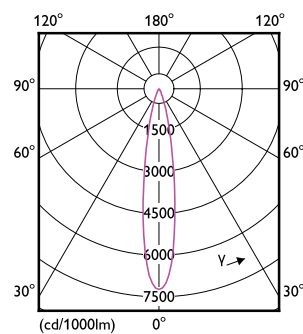
Light Distribution Diagram - RS350 G2 RC Rd D75 11W 27K 15D 1H
