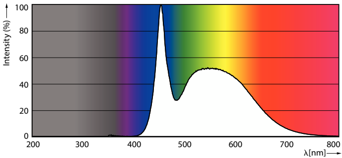
Spectral Power Distribution Colour - LED MOD 14W 865
