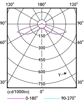
Light Distribution Diagram - LED MOD 14W 865
