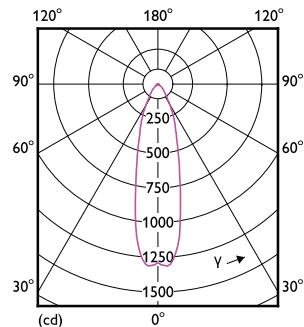
Light Distribution Diagram - MAS LEDspot VLE D 6-50W 940 PAR20 25D
