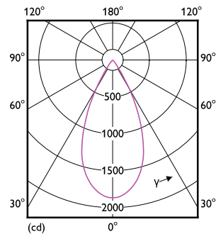
Light Distribution Diagram - RS350 G2 RC Rd D75 11W 40K 50D 1H
