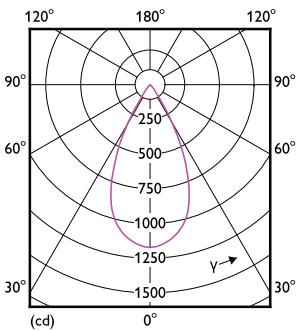
Light Distribution Diagram - RS350 G2 RC Rd D75 9W 30K 50D 1H
