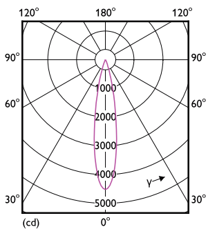
Light Distribution Diagram - RS350 G2 RC Rd D75 7W 40K 24D 1H
