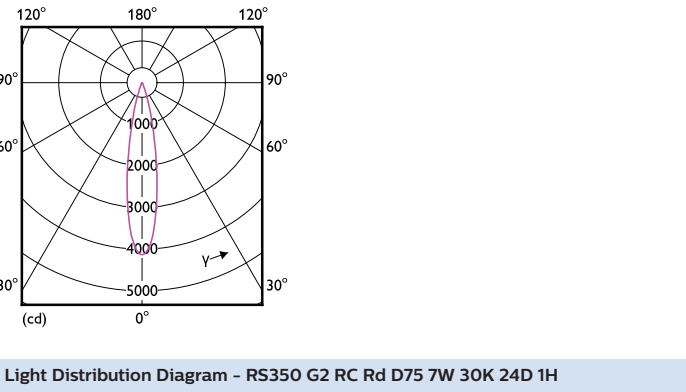
Light Distribution Diagram - RS350 G2 RC Rd D75 7W 30K 24D 1H
