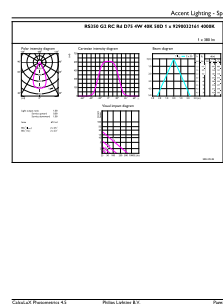
Accent Lighting Spots - RS350 G2 RC Rd D75 4W 40K 50D 1H
