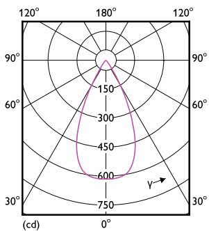
Light Distribution Diagram - RS350 G2 RC Rd D75 4W 40K 50D 1H
