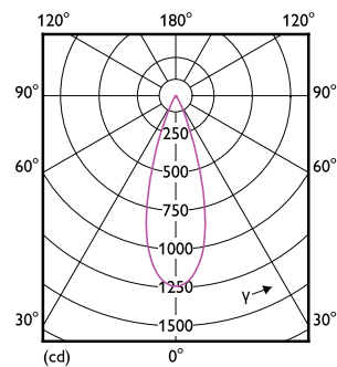
Light Distribution Diagram - RS350 G2 RC Rd D75 4W 40K 36D 1H
