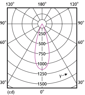
Light Distribution Diagram - RS350 G2 RC Rd D75 4W 30K 36D 1H
