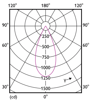
Light Distribution Diagram - RS350 G2 RC Rd D55 7W 40K 50D 1H
