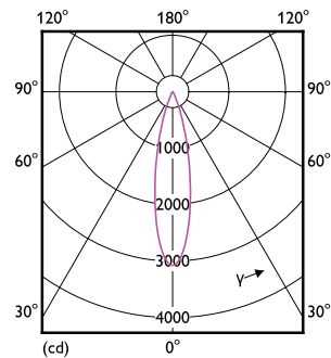
Light Distribution Diagram - RS350 G2 RC Rd D55 7W 40K 24D 1H
