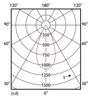
Light Distribution Diagram - RS350 G2 RC Rd D55 7W 30K 50D 1H
