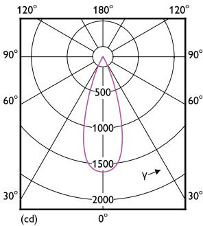
Light Distribution Diagram - RS350 G2 RC Rd D55 7W 30K 36D 1H
