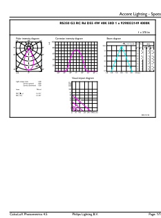
Accent Lighting Spots - RS350 G2 RC Rd D55 4W 40K 50D 1H
