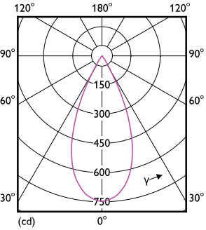
Light Distribution Diagram - RS350 G2 RC Rd D55 4W 40K 50D 1H
