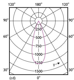
Light Distribution Diagram - RS350 G2 RC Rd D55 4W 40K 36D 1H
