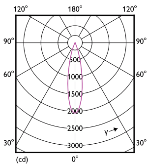
Light Distribution Diagram - RS350 G2 RC Rd D55 4W 40K 24D 1H
