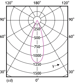
Light Distribution Diagram - RS350 G2 RC Rd D55 4W 30K 36D 1H
