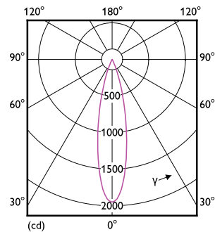
Light Distribution Diagram - RS350 G2 RC Rd D55 4W 30K 24D 1H
