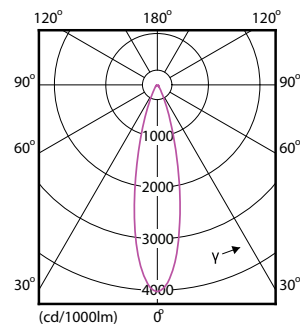
Light Distribution Diagram - Mag Spotlight 6.5W 530lm 30K 24D
