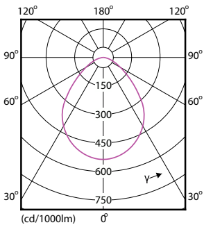
Light Distribution Diagram - Mag L Flood 12.5W 1100lm 40K
