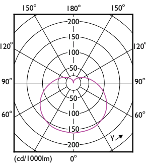
Light Distribution Diagram - LEDBulb 12W B22 965 230V 1PF/6 AU
