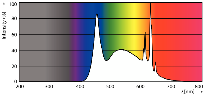
Spectral Power Distribution Colour - LEDBulb 12W B22 965 230V 1PF/6 AU
