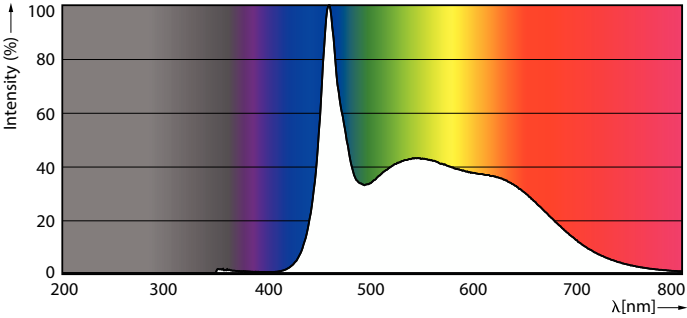
Spectral Power Distribution Colour - LEDBulb 12W E27 965 230V 1PF/6 AU
