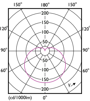
Light Distribution Diagram - LEDBulb 12W B22 930 230V 2PF/3 AU
