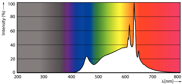
Spectral Power Distribution Colour - LEDBulb 12W B22 930 230V 2PF/3 AU
