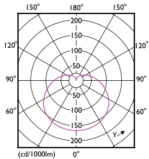
Light Distribution Diagram - LEDBulb 10W B22 965 230V 1PF/6 AU
