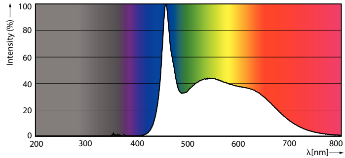
Spectral Power Distribution Colour - LEDBulb 10W E27 965 230V 1CT/12 CN
