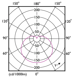
Light Distribution Diagram - LEDBulb 10W E27 965 230V 1CT/12 CN
