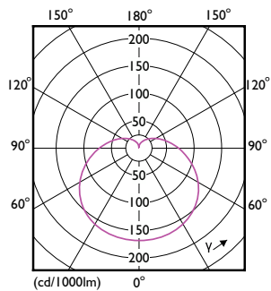
Light Distribution Diagram - LEDBulb 10W B22 930 230V 1PF/6 AU
