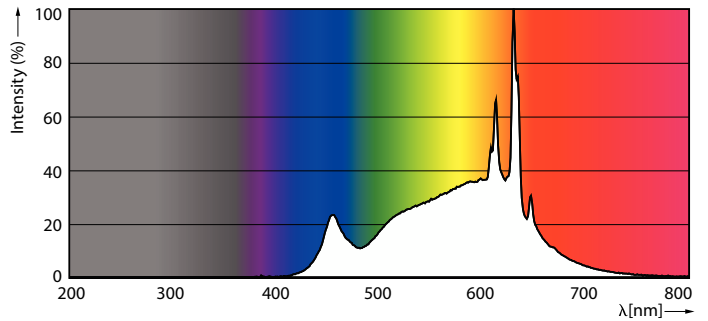
Spectral Power Distribution Colour - LEDBulb 10W B22 930 230V 1PF/6 AU
