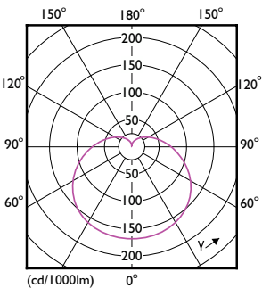
Light Distribution Diagram - LEDBulb 10W B22 930 230V 1PF/6 AU
