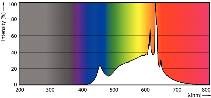
Spectral Power Distribution Colour - LEDBulb 10W B22 930 230V 1PF/6 AU
