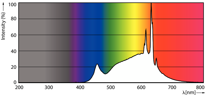
Spectral Power Distribution Colour - LEDBulb 10W B22 930 230V 2PF/3 AU
