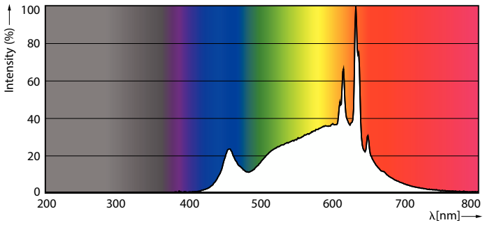
Spectral Power Distribution Colour - LEDBulb 10W E27 930 230V 1PF/6 AU
