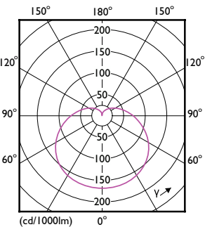
Light Distribution Diagram - LEDBulb 10W E27 930 230V 1PF/6 AU
