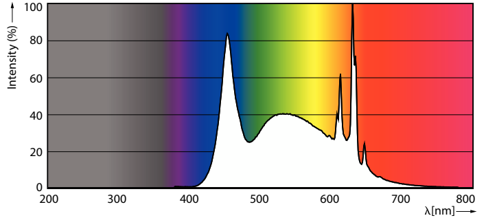
Spectral Power Distribution Colour - LEDBulb 8W B22 965 230V 1PF/6 AU
