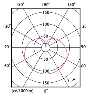
Light Distribution Diagram - LEDBulb 8W E27 965 230V 1PF/6 AU
