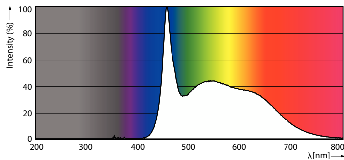
Spectral Power Distribution Colour - LEDBulb 8W E27 965 230V 1PF/6 AU
