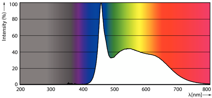
Spectral Power Distribution Colour - LEDBulb 8W E27 965 230V 2PF/3 AU
