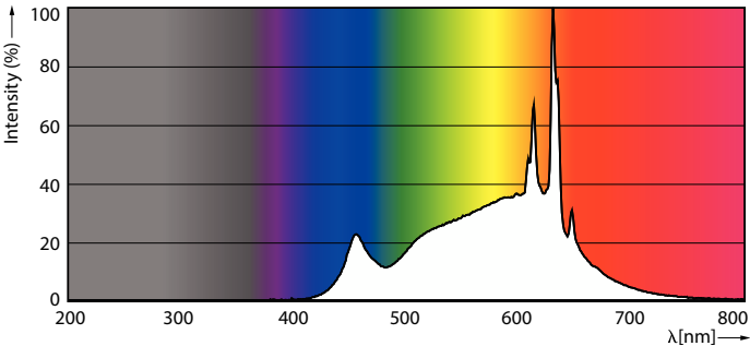
Spectral Power Distribution Colour - LEDBulb 8W B22 930 230V 1PF/6 AU
