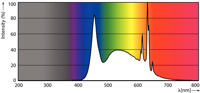
Spectral Power Distribution Colour - LEDBulb 6W B22 965 230V 1PF/6 AU
