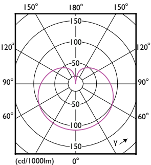
Light Distribution Diagram - LEDBulb 6W E27 965 230V 1PF/6 AU
