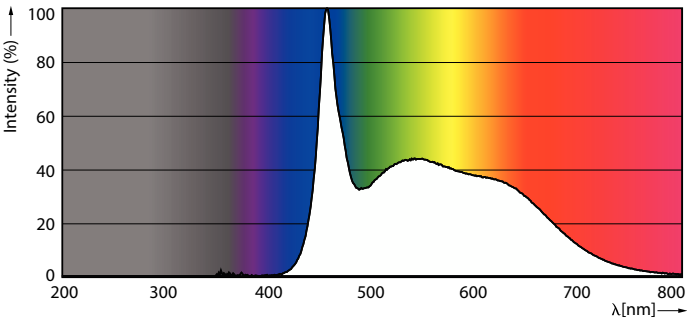
Spectral Power Distribution Colour - LEDBulb 6W E27 965 230V 1PF/6 AU
