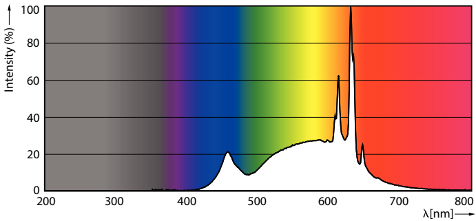
Spectral Power Distribution Colour - LEDBulb 6W E27 930 230V 2PF/3 AU
