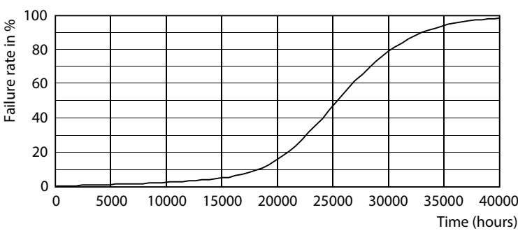
L70B-50 25K-LED
