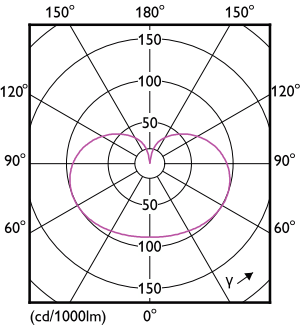
Light Distribution Diagram - LED Sensor 8-60W B22 CDL FR 1PF/6 APR
