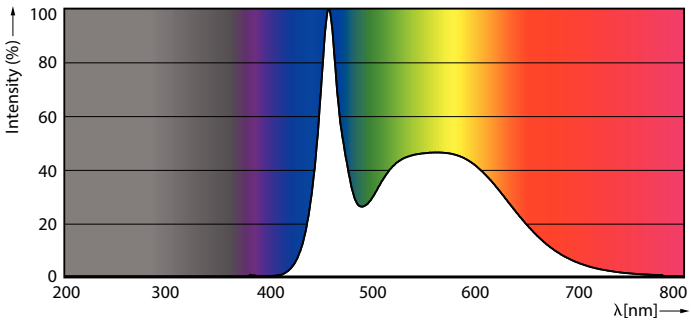
Spectral Power Distribution Colour - LED Sensor 8-60W B22 CDL FR 1PF/6 APR
