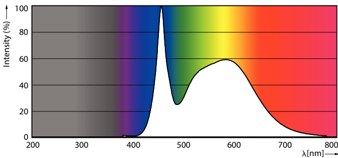
Spectral Power Distribution Colour - 29A21/PER/850/FR/P/E26/D/HO 4/1PF
