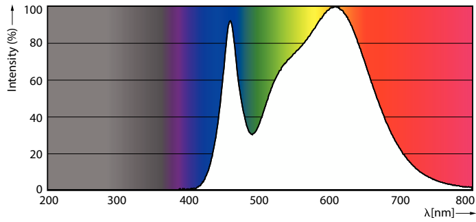
Spectral Power Distribution Colour - ESS LEDBulb 9W E27 4000K 230V 1CT/12 CN
