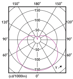
Light Distribution Diagram - ESS LEDBulb 9W E27 4000K 230V 1CT/12 CN
